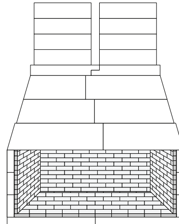
FULLY BRICKED FIREBOX COVERING EXPANSION GAPS
