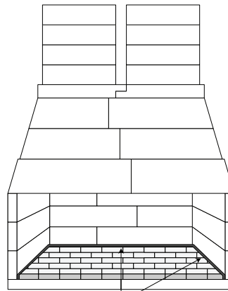
FLOOR WITH 1/2" EXPANSION GAP ALONG BACK AND SIDE WALLS
