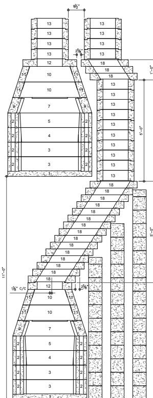
FIGURE 10.4 INSTALLATION WITH OFFSET BLOCKS (SEE FIGURE 15 ON PAGE 33 FOR MORE DETAILS)
