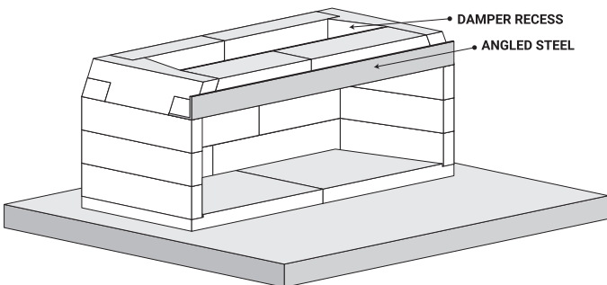
FIGURE 7.3 DAMPER RECESS + ANGLED STEEL
