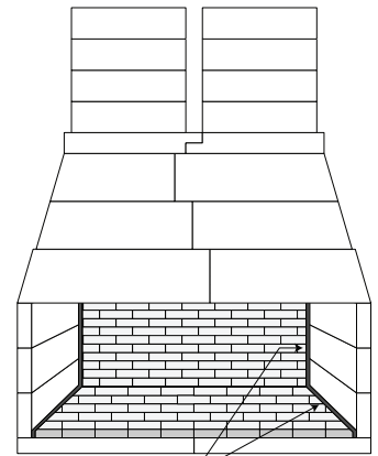
FLOOR & BACK WALL WITH 1/2" EXPANSION GAP ALONG SIDE WALLS
