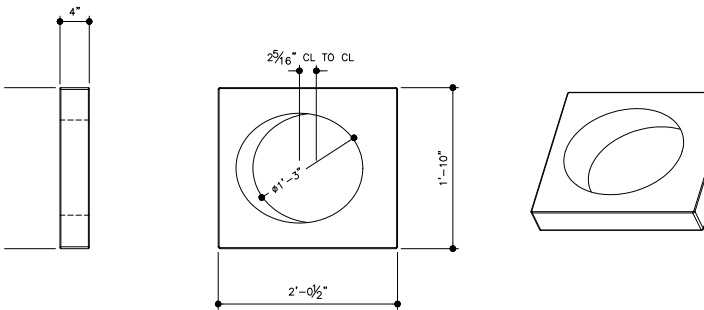
FIGURE 10.3 OFFSET BLOCK
