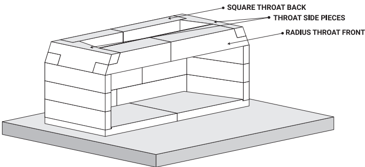
FIGURE 7.2 ASSEMBLED THROAT
